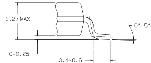
DETAIL A TYPICAL
